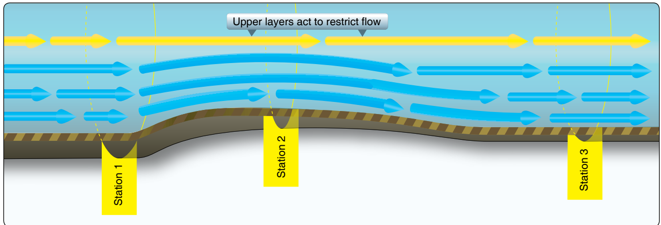
Figure 2-7. Venturi flow.
