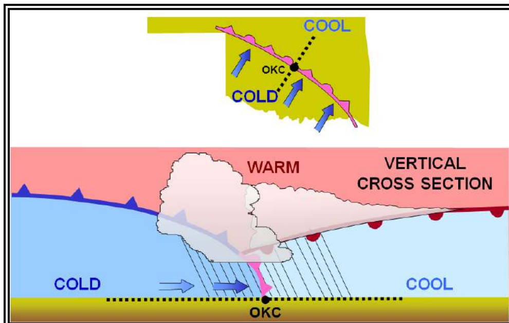
Figure 10-8. Occluded Front
