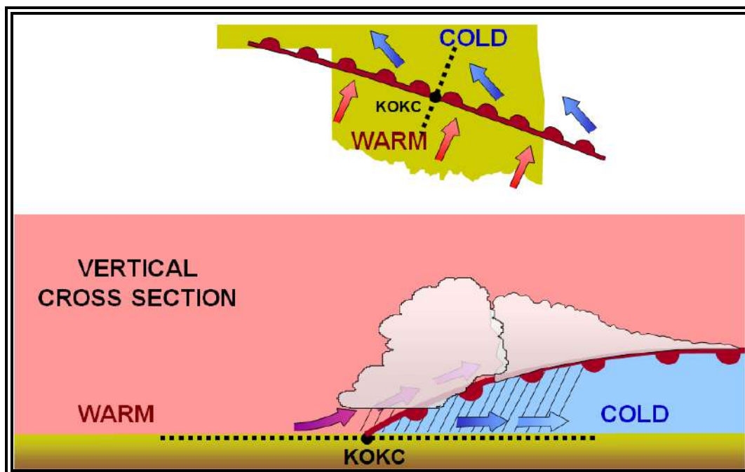
Figure 10-6. Warm Front
