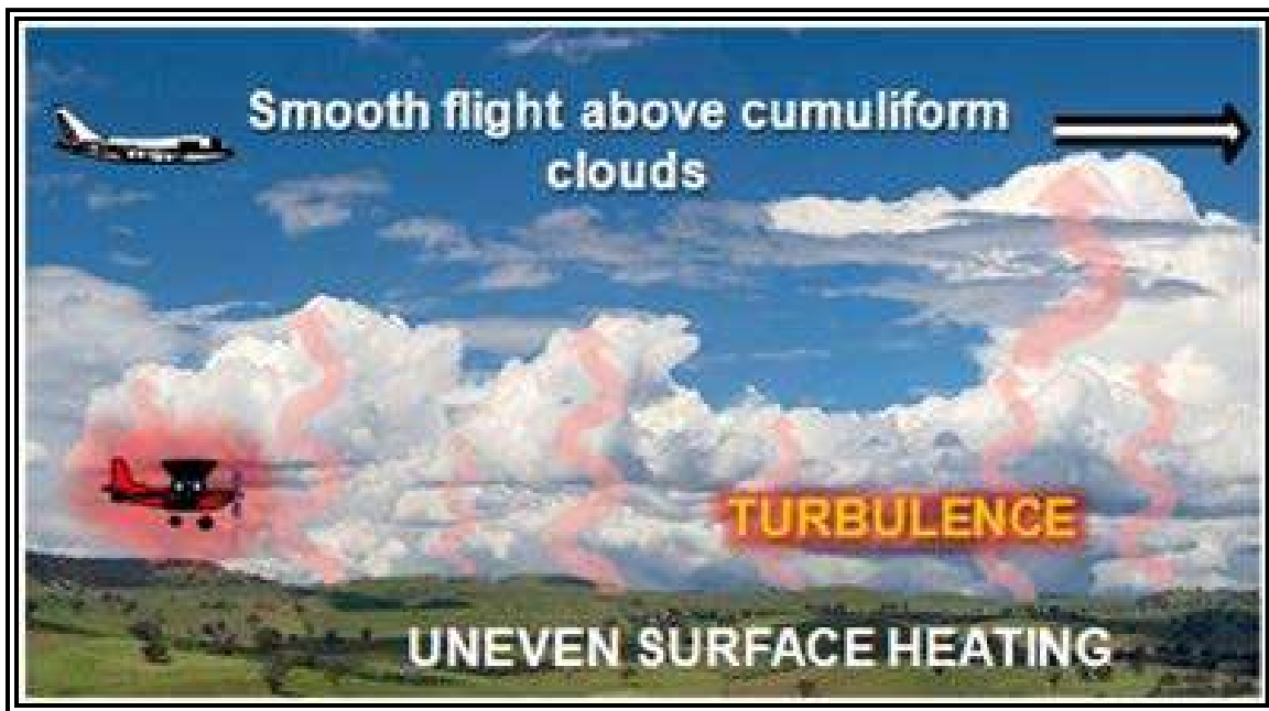
Figure 17-1. Convective Turbulence
