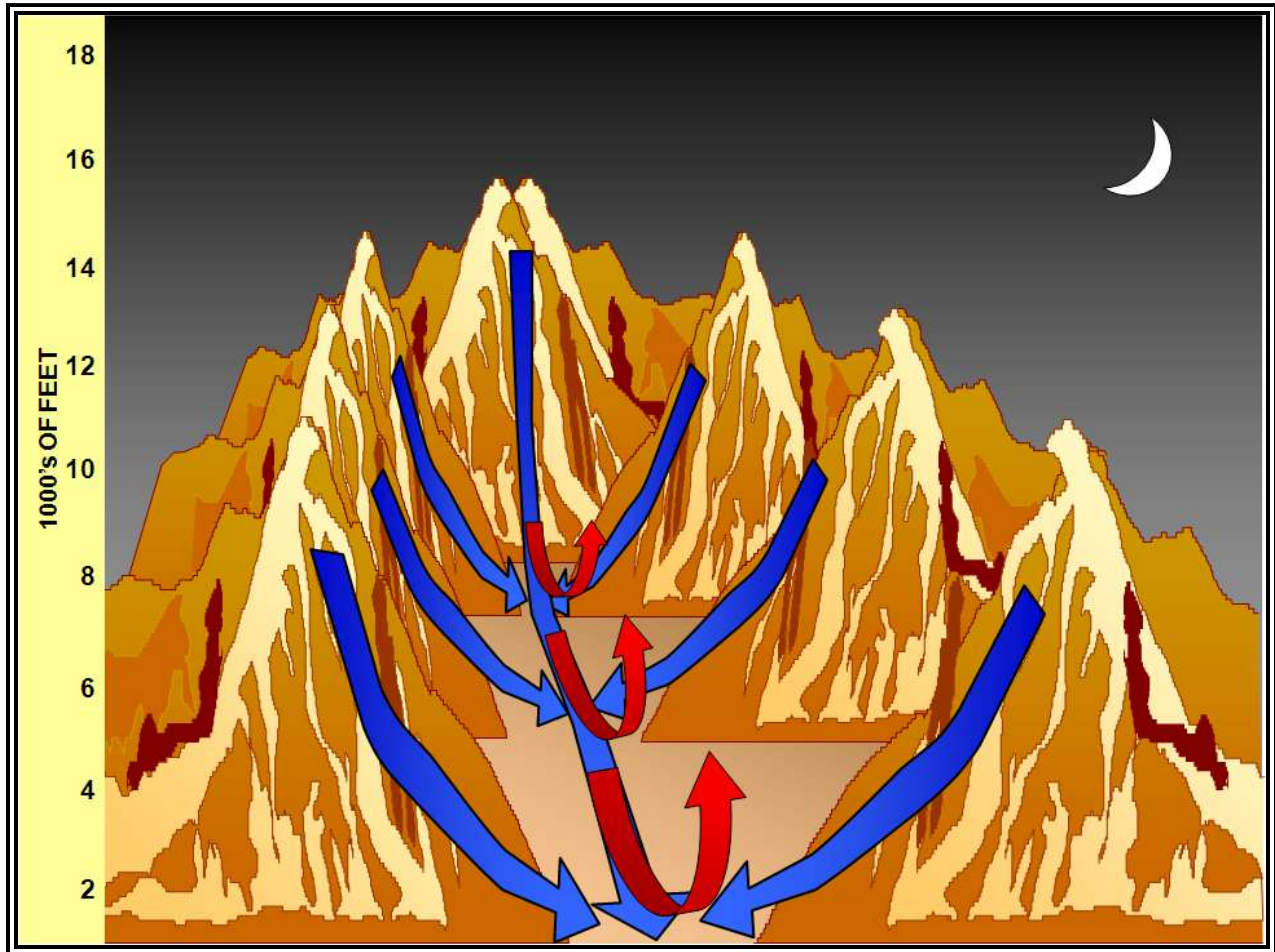
Figure 9-10. Mountain Breeze
