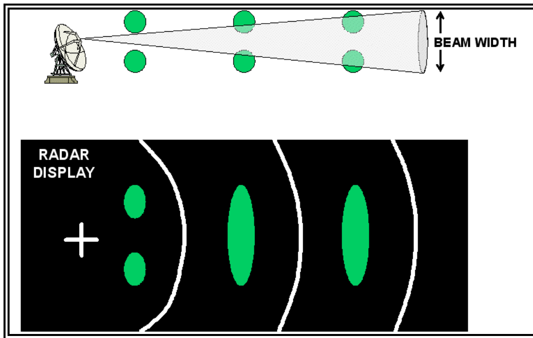
Figure 20-6. Beam Resolution
