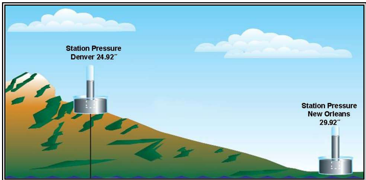
Figure 5-3. Station Pressure
