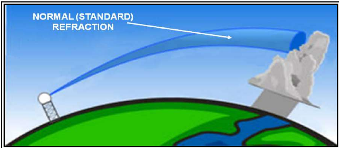
Figure 20-8. Normal Refraction
