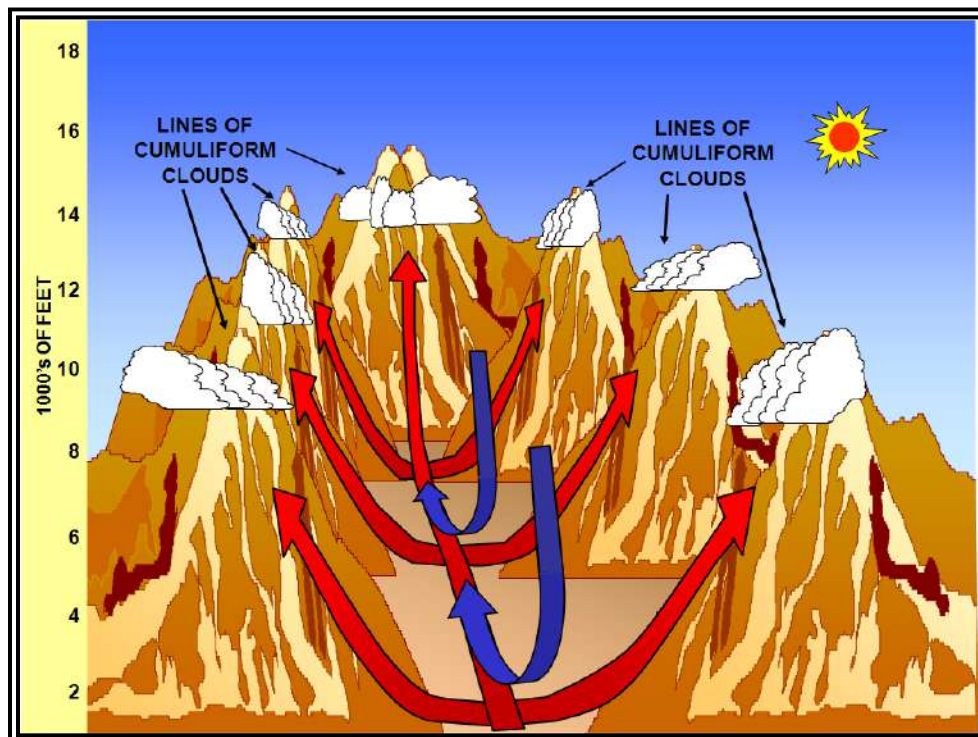
Figure 9-8. Valley Breeze
