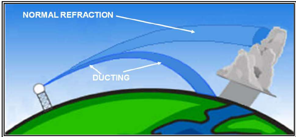
Figure 20-11. Ducting
