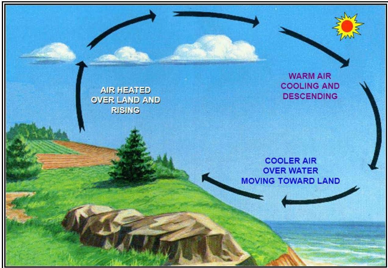
Figure 9-2. Sea Breeze
