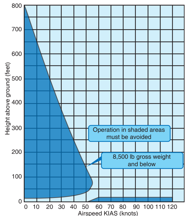
Figure 10-10. Height/velocity chart.
