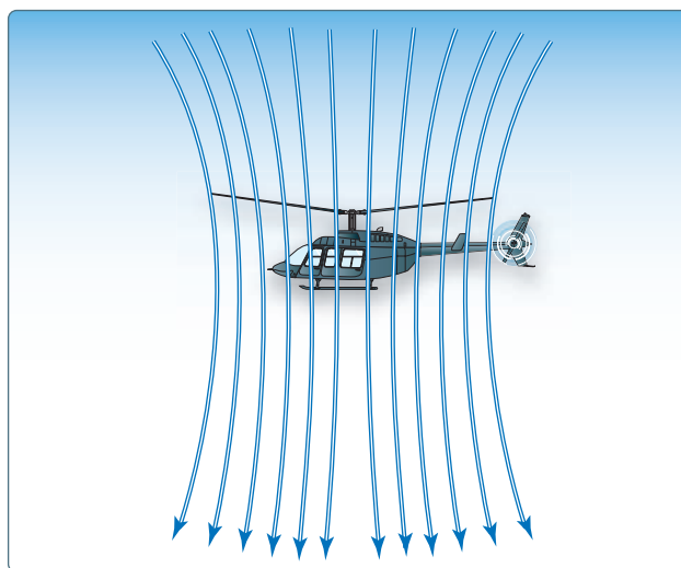
Figure 2-15. Induced flow.
