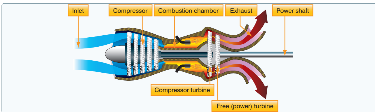
Figure 7-26. Turboshaft engine.
