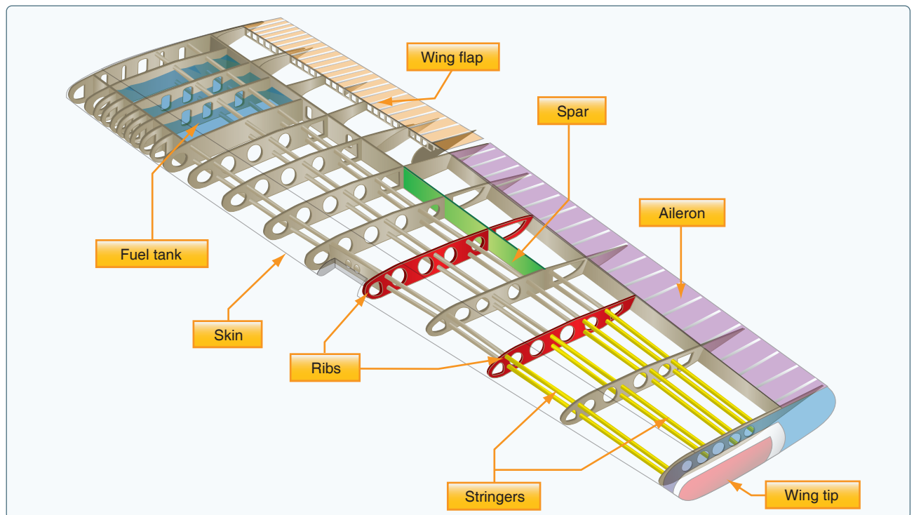
Figure 3-7. Wing components.
