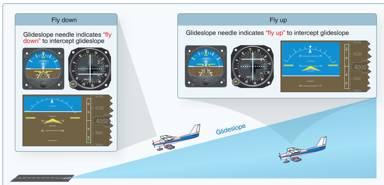
Figure 3-22. Analog and digital indications for glideslope interception.
