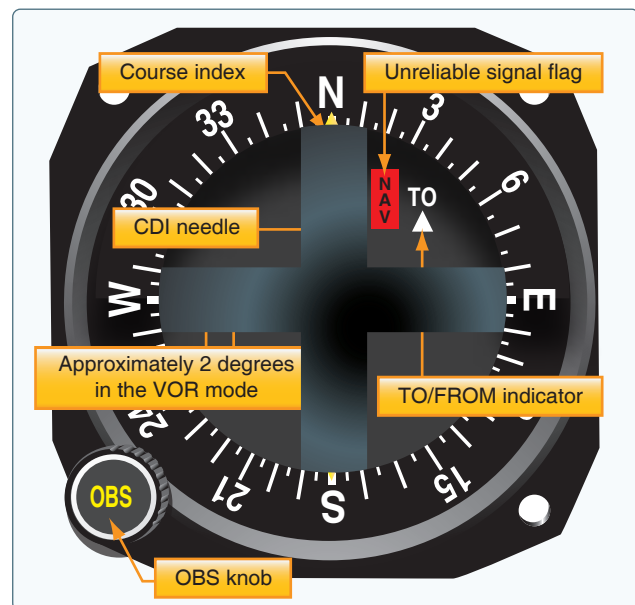
Figure 16-29. VOR indicator.
