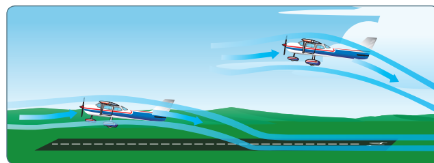
Figure 5-16. Ground effect changes airflow.
