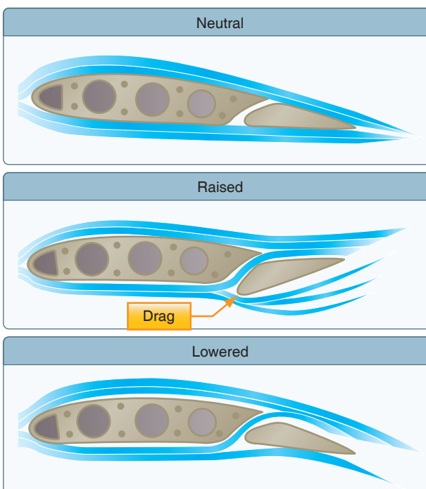
Figure 6-7. Frise-type ailerons.
