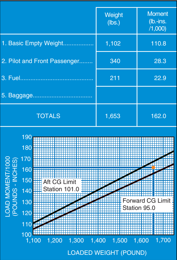
Figure 7-8. CG/Moment Chart.
